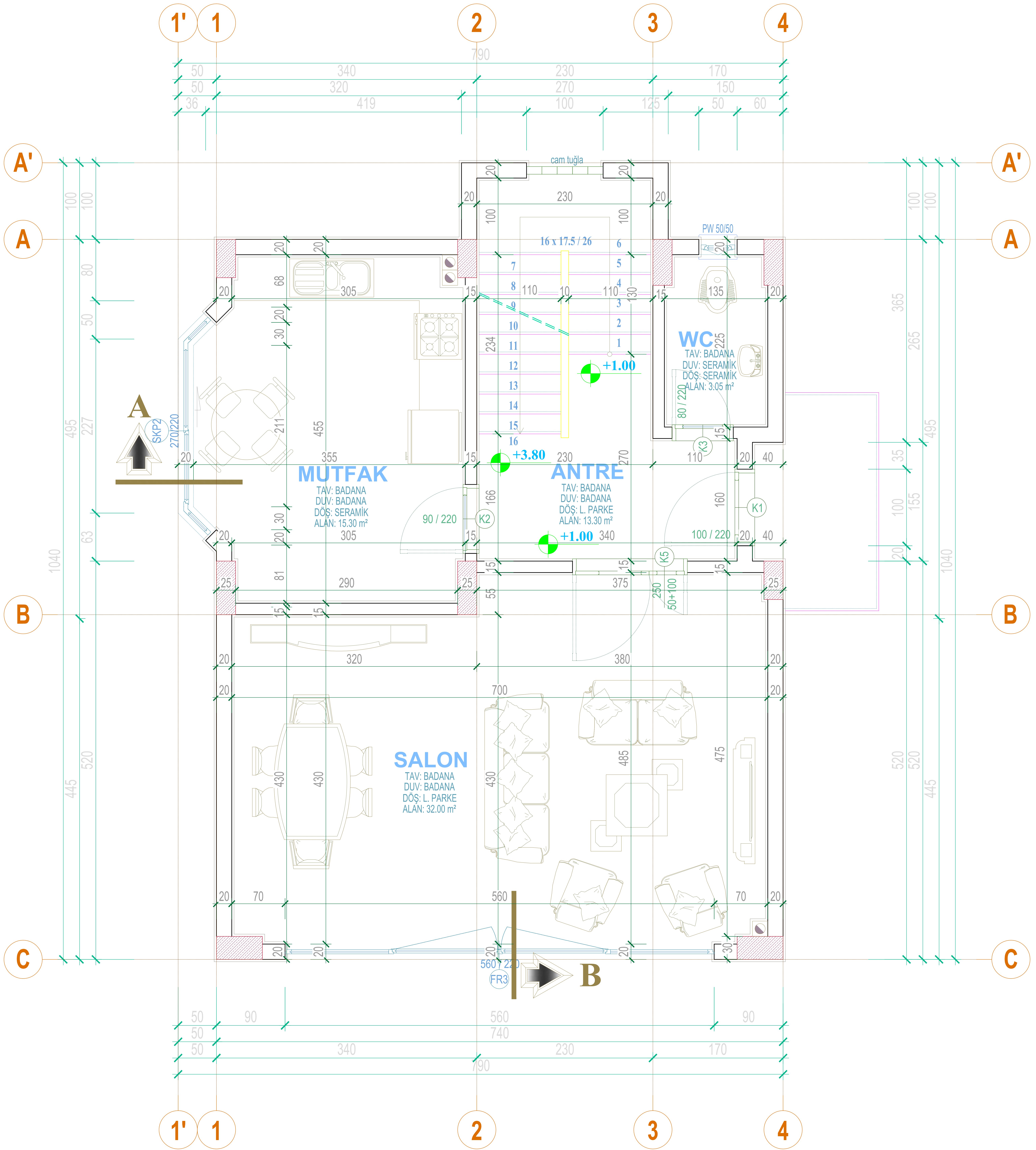
ZEMİN KAT PLANI 1 / 50
